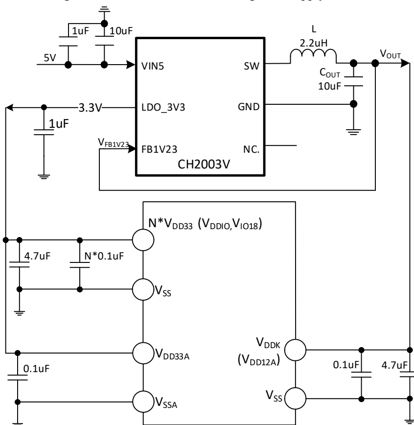
Figure 3-1-6 CH32H415 DCDC single 5V supply circuit
