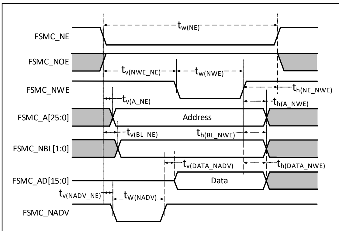
Figure 3-17-2 Asynchronous bus non-multiplexing PSRAM/NOR write operation waveform
