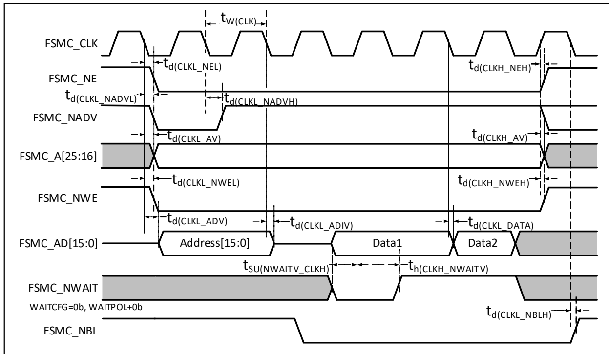
Figure 3-19 Synchronous bus multiplexing PSRAM write waveforms
