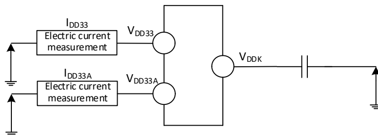
Figure 3-2-3 CH32H415 Current consumption measurement
