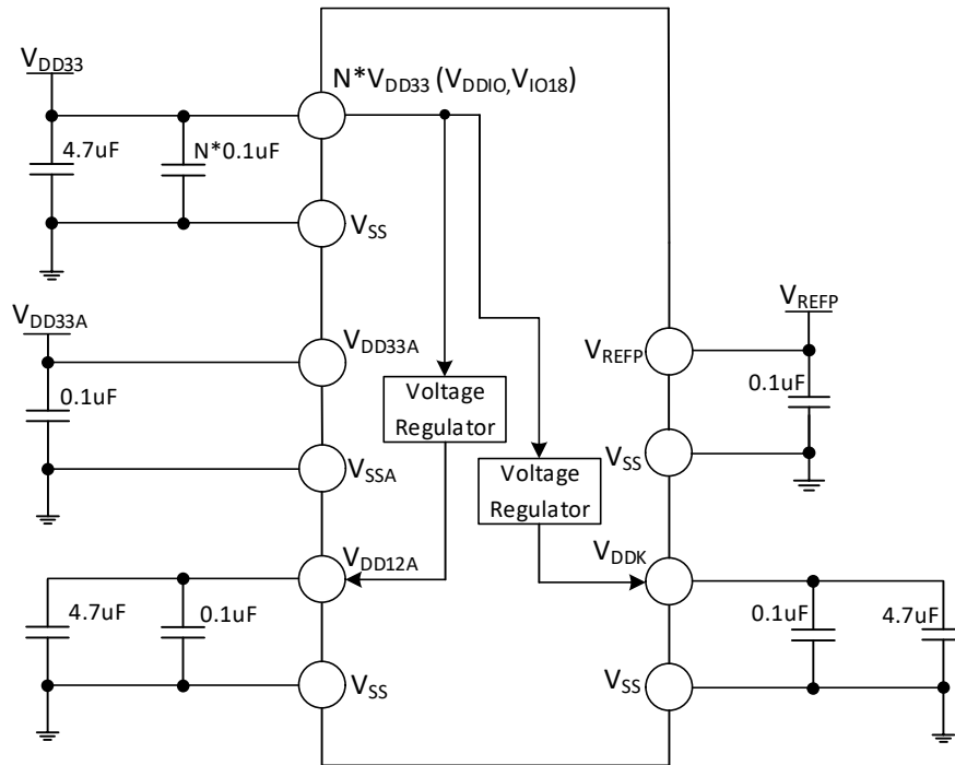
Figure 3-1-3 CH32H416 Conventional power supply typical circuit
