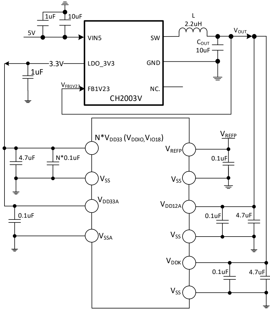
Figure 3-1-4 CH32H416 DCDC single 5V supply circuit
