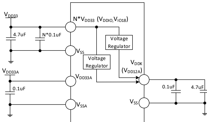
Figure 3-1-5 CH32H415 Conventional power supply typical circuit
