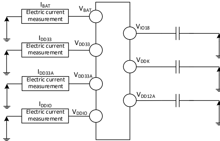
Figure 3-2-1 CH32H417 Current consumption measurement
