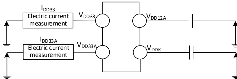
Figure 3-2-2 CH32H416 Current consumption measurement
